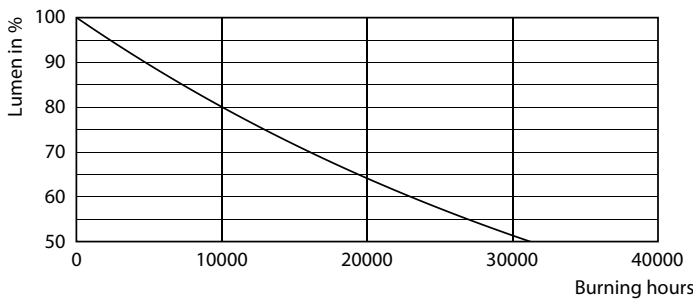
Lumen Maintenance Diagram - LED classic 150W A67 E27 CDL FR ND 1SRT4
