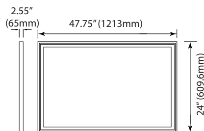
P10098 MT-2x4BOX (2 x 4 Surface Mount Kit)
