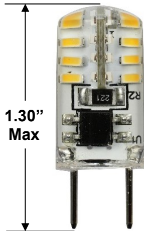
G-8 Base (8mm Pin Centers)
