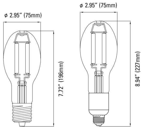
ED23.5 Lamp 20 Watt: 0.37-lb
