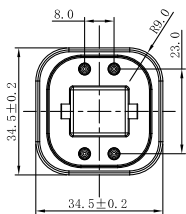
SubstiTUBE UL Type A Base – G24q
