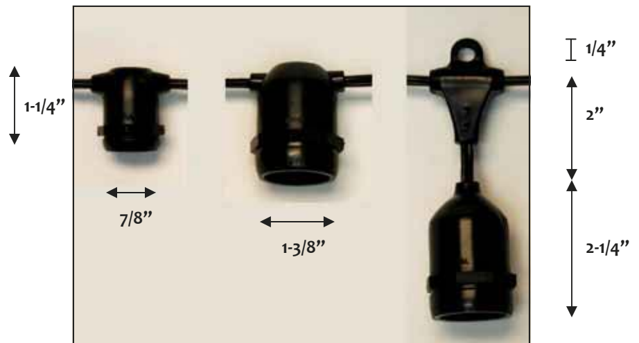
Intermediate Base In-line Socket (see pg. 28)
