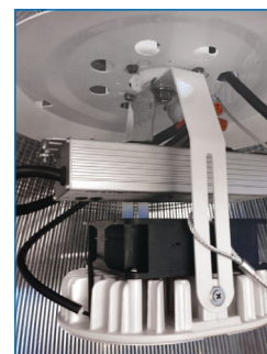
A retrofit LED lamp and driver installed inside a high-bay fixture
