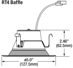
RT4 Baffle
