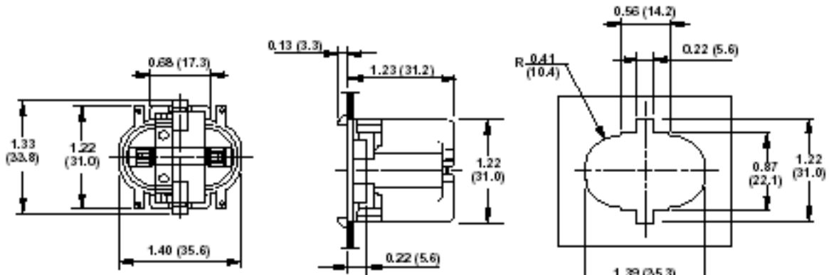
PANEL CUTOUT,
