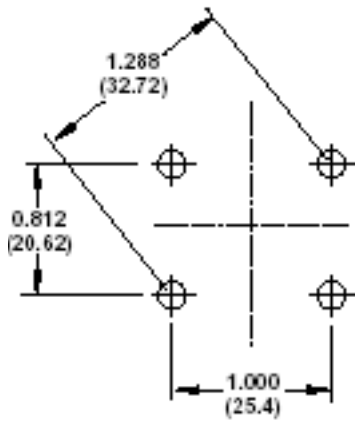
RECOMMENDED HOLE PATTERN
