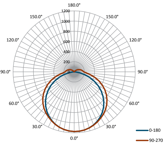
2ft Luminaire, 120V, 30W, 3500K
