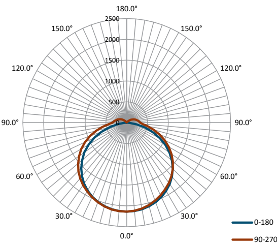
4ft Luminaire, 120V, 60W, 3500K
