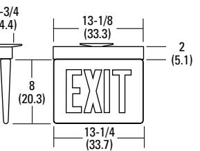
Top Mount (AC only operation)
