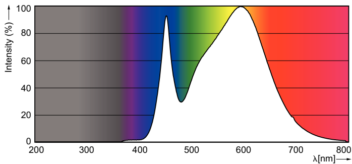
20-100W AR111 /840
