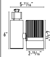
Dimensions For L4 & 16° Optic
