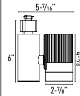
Dimensions For L3
