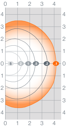
30W fixture at 15' mounting height
