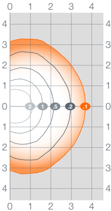
20W fixture at 15' mounting height
