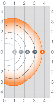
10W fixture at 10' mounting height
