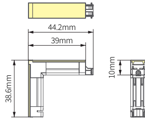
*Corner Out Connector
