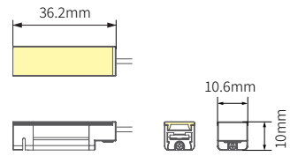
*Shortest Fixture(38mm) with Power Cable
