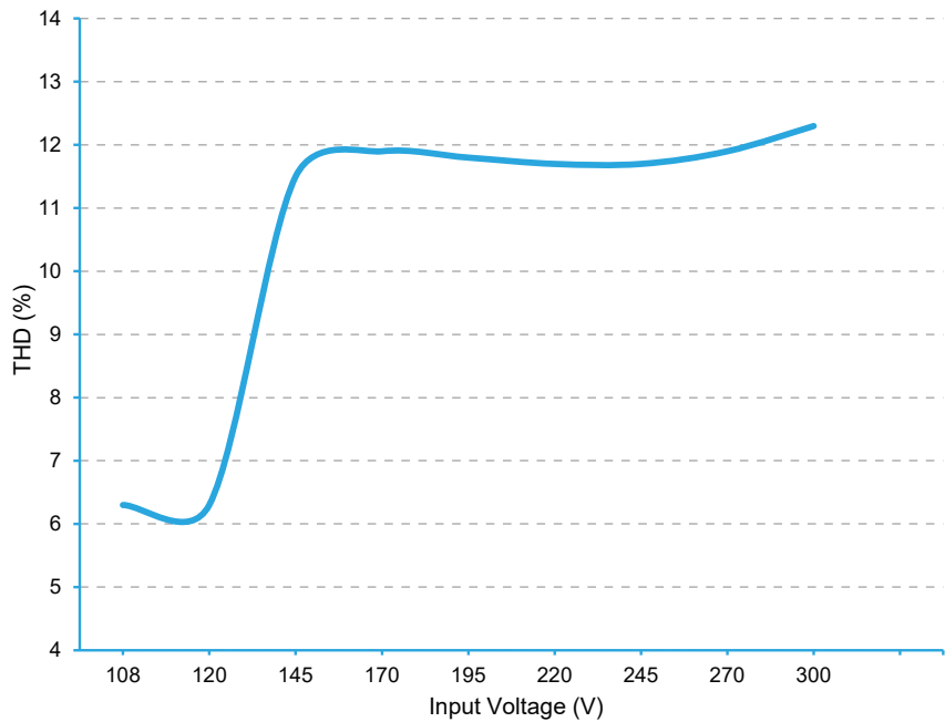
THD vs. Input Voltage (Full Load)
