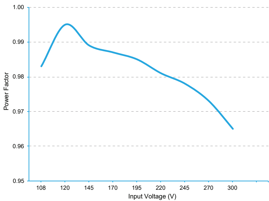
Power Factor vs. Input Voltage (Full Load)
