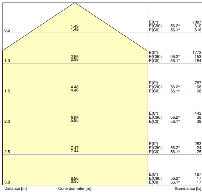
PL PROT 600 P 22W 840 PS 3080lm
