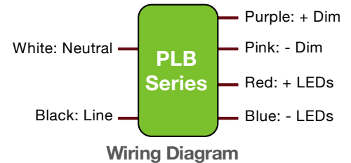
Flying Leads Case L 198.7 * W 18.25 * H 18.25 mm (L 7.82 * W 0.72 * H 0.72 in.)
