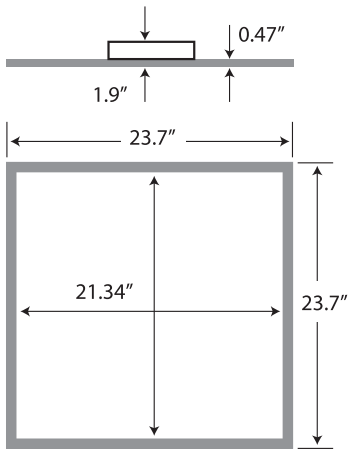
40W 2x2 LED Panel
