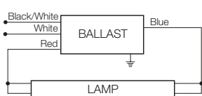
QUICKTRONIC 1x32
