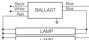
QUICKTRONIC 2x32
