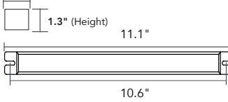
45W DRIVER
