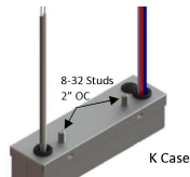
K Case 4.07" L X 1.03" W X 0.94" H
