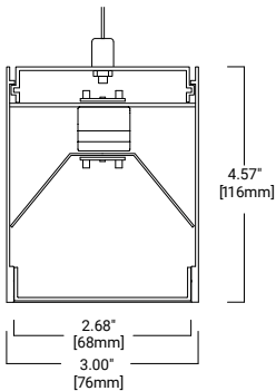
Standard Housing
