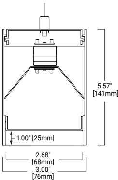
Regressed Housing
