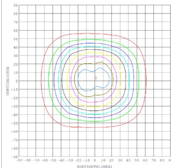
Isocandela (Rectangle)
