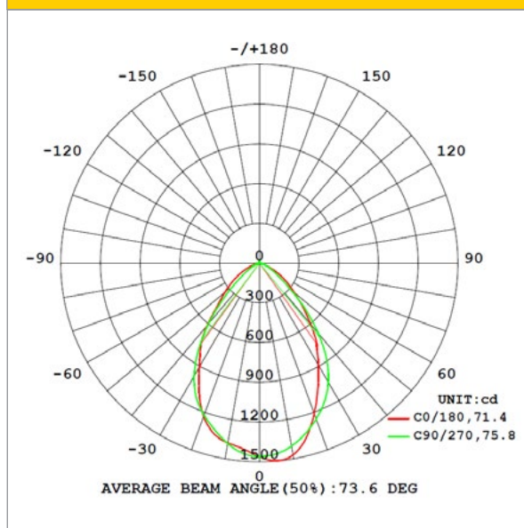
LPF1-15, 15W at 75°
