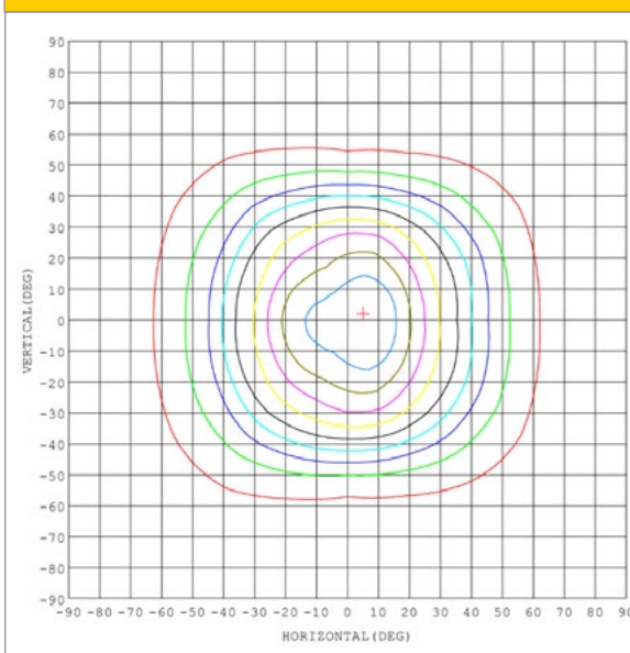
Isocandela (Rectangle)
