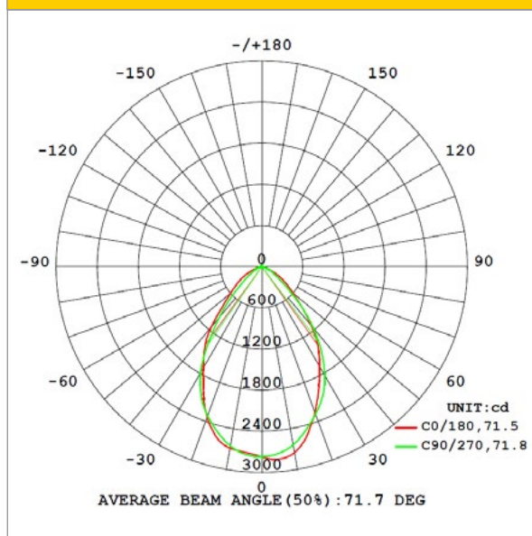
LPF1, 30W at 75°
