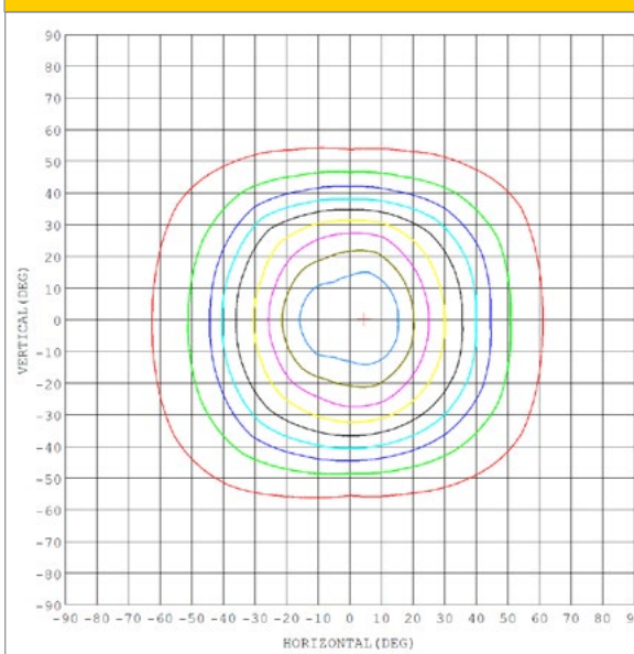
Isocandela (Rectangle)
