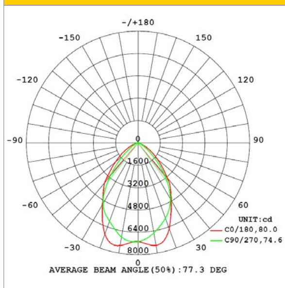
LPF2-H 80W at 75°
