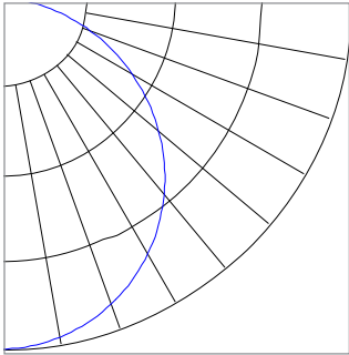
SLM22-PS40 / FCCT (Typical performance @ 40W, 4000K)
