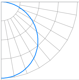
SLM22-44/B0/8xx (Typical performance @ 4000K)
