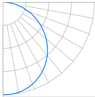
SLM24-44/B0/8xx (Typical performance @ 4000K)
