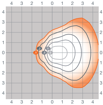
SLIMWP2AS60UNH-25FT with 30° tilt
