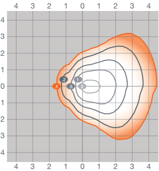
SLIMWP2AS30UNH-20FT with 30° tilt
