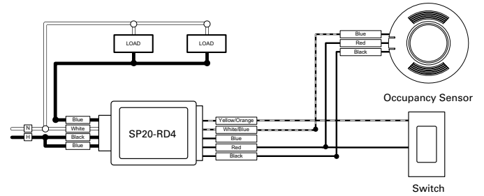
Manual ON/Auto OFF with Local Switch
