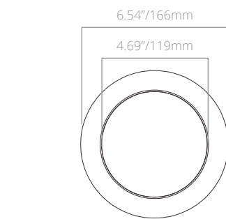
6" Trim Ring
