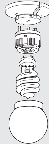
SpringLamp® Keyless Fixture
