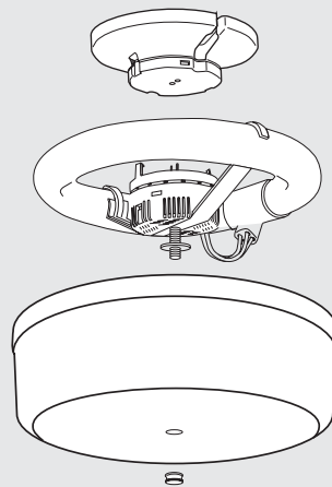
Circline Keyless Fixture
