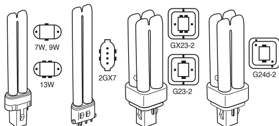
G23 base Twin Tube
