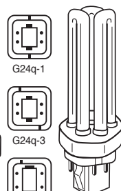
G24q-2 (DBX4P) GX24q base Triple Tube
