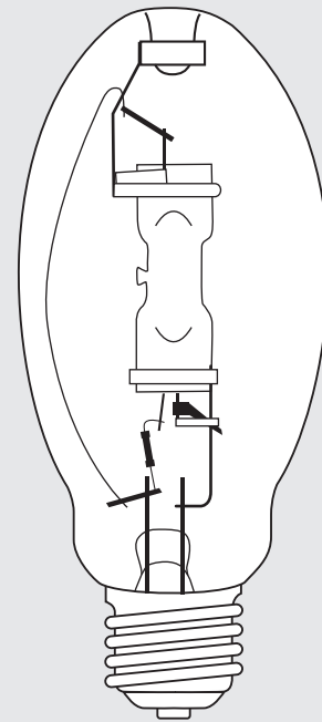
ED28 Mogul Base Enclosed Rated
