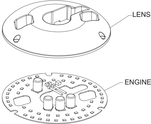
Exploded View
