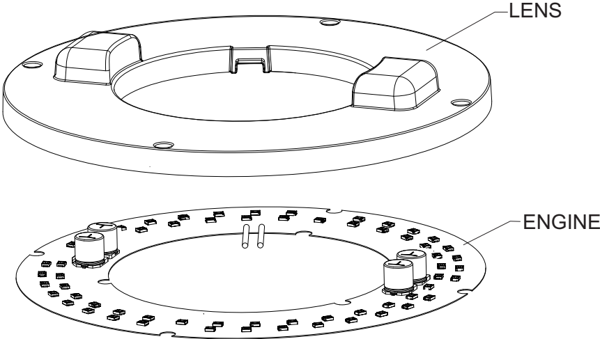
Exploded View
