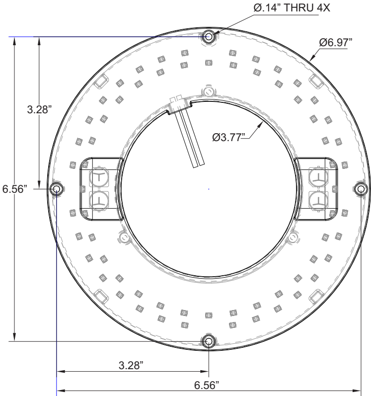
Top View
