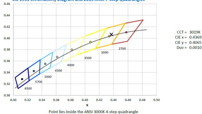
CIE 1931 Chromaticity Diagram and 2015 ANSI 7-Step Quadrangles
