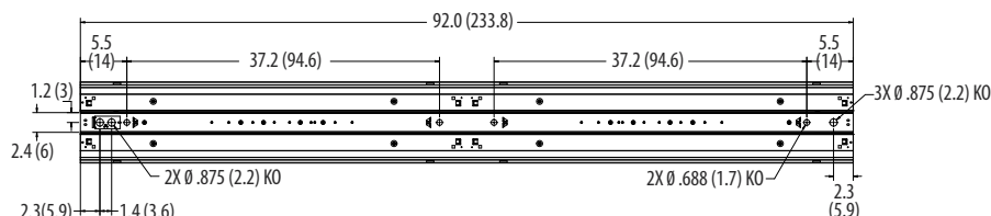
UFIT L92 KEY DIMENSIONS
