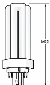
(6) 4-Pin Base
