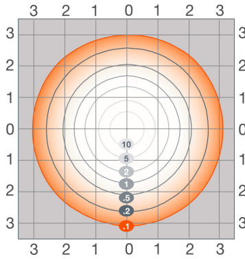
Isofootcandle Lines at 20' Mounting Height
