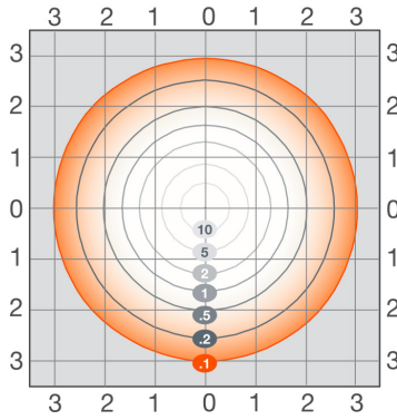
Isofootcandle Lines at 30' Mounting Height
