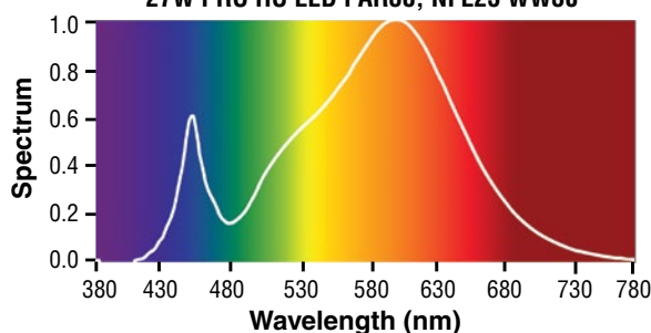
Item 1005039 27W PRO HO LED PAR38, NFL25 WW30
