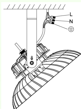
Adjustable Surface Mounting
