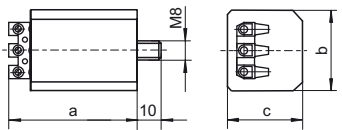
PC casing
