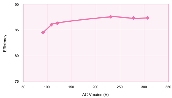
Efficiency vs. Vmains
