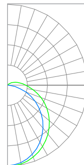
VTS4 / PS60 / 8xx / UD (Typical performance @60W, 4000K)
