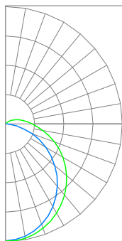
VTS4 / PS60 / FCCT / UD (Typical performance @60W, 4000K)
