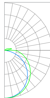
VTS8 / PS100 / 8xx / UD (Typical performance @100W, 4000K)
