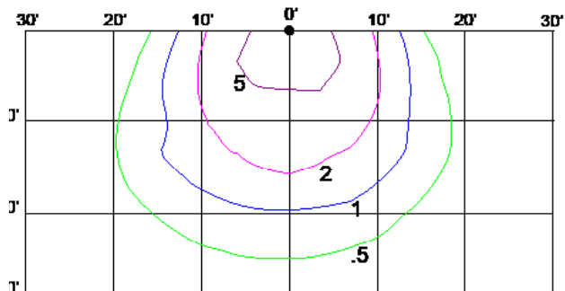
28W 3,640 LUMENS 10' MOUNTING HEIGHT
