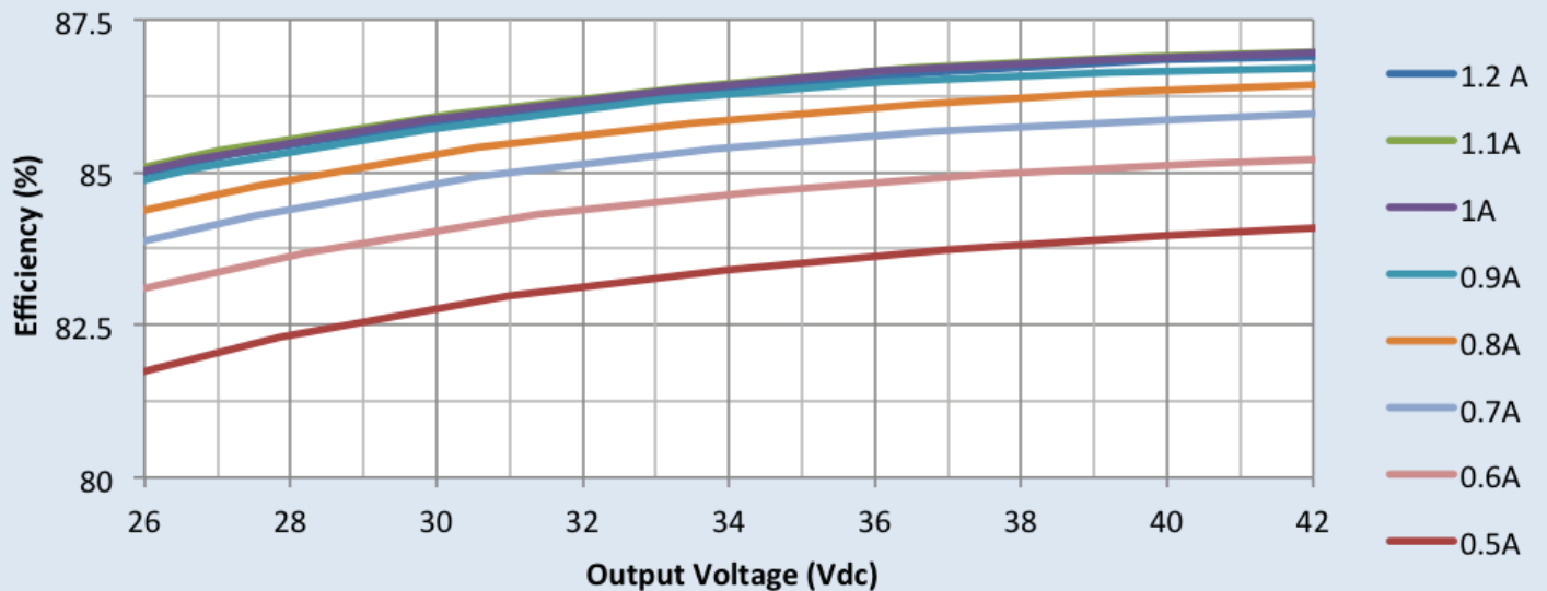
Efficiency vs. Output Voltage at 120Vac @ T c =70°C
