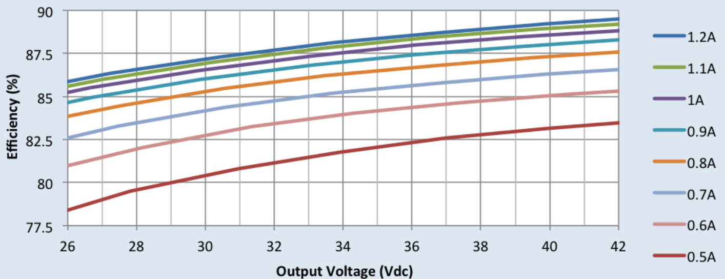
Efficiency vs. Output Voltage at 277Vac @ T c =70°C
