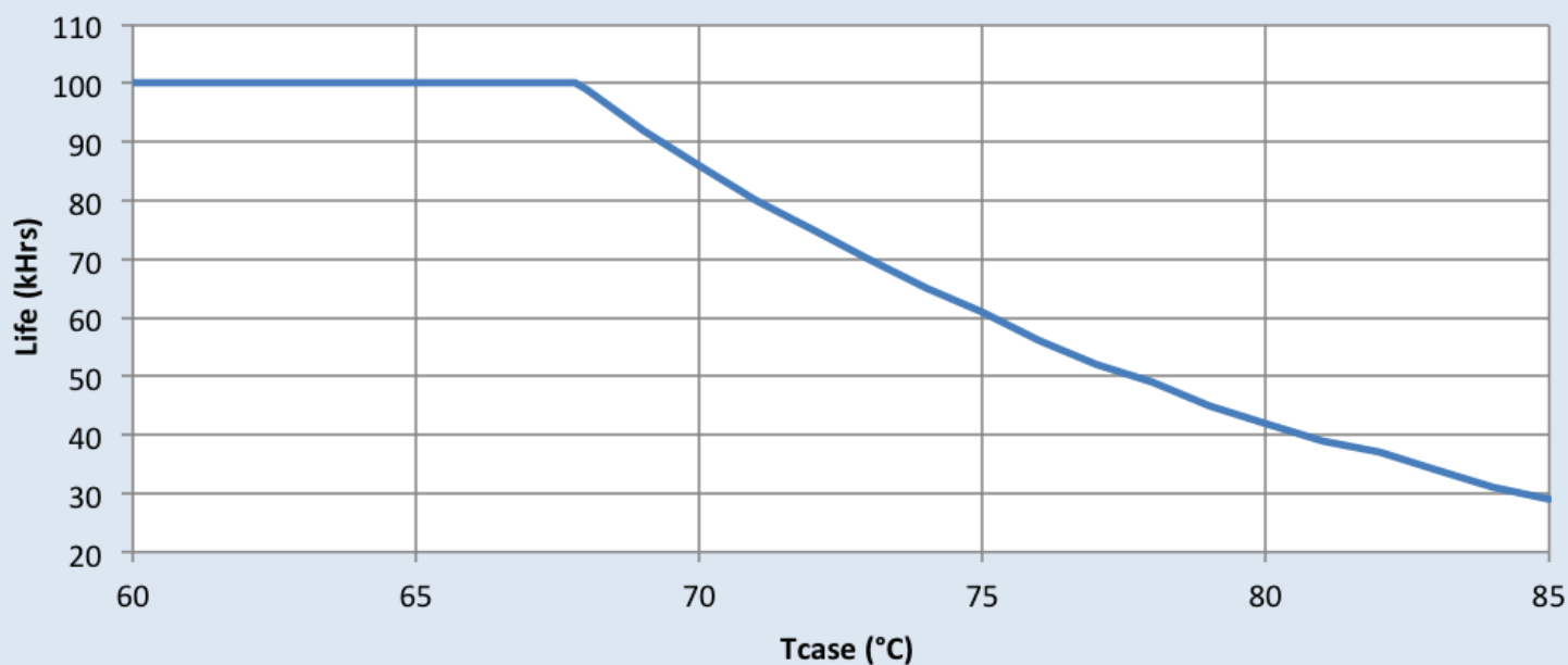
Lifetime vs. Tcase
