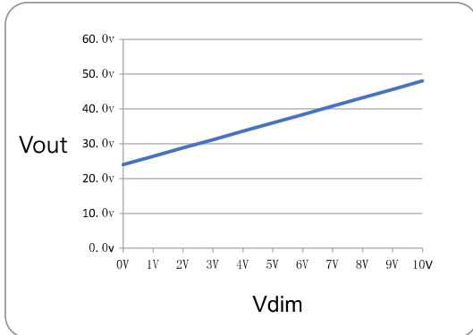
Dimming Curve
